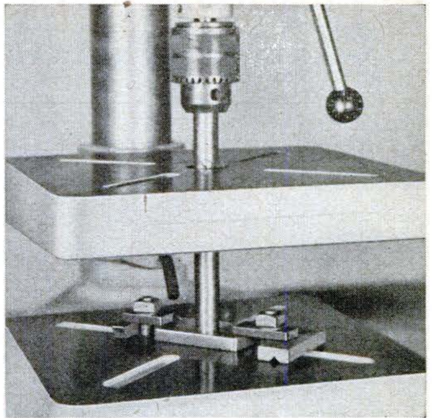
This boring setup enlarges the center hole of the drill-press table. Note the lower bearing.
